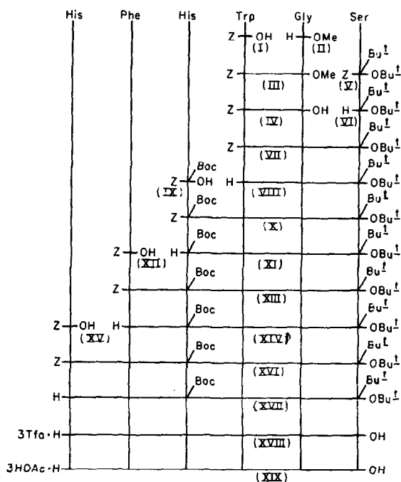
FIG. 1. Synthesis of the hexapeptide L-histidyl-L-phenylalanyl-L-histidyl-L-tryptophanyl-glycyl-L-serine.
